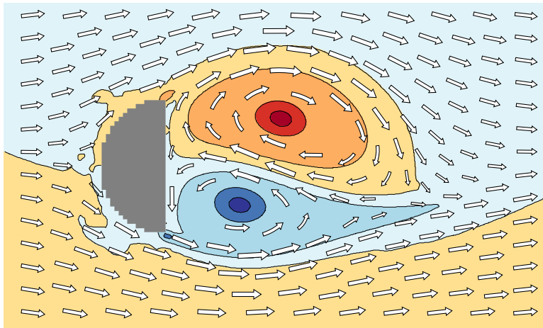
Figure 1: Vortex sheet detachment in flow around a half-cylinder, background is vorticity, data by gerris 1.1.2, arrows by vplot 0.9.3
